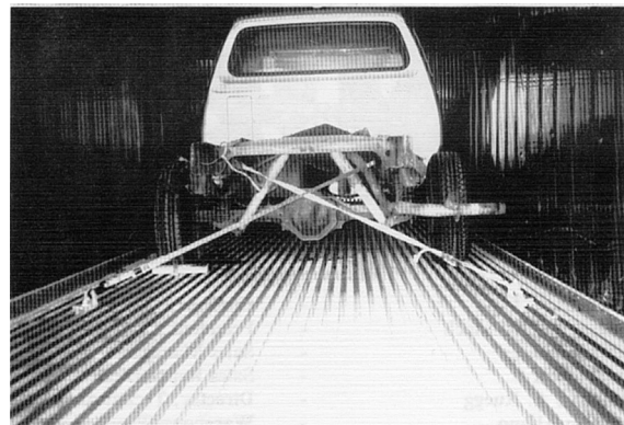
Wheel Chock
