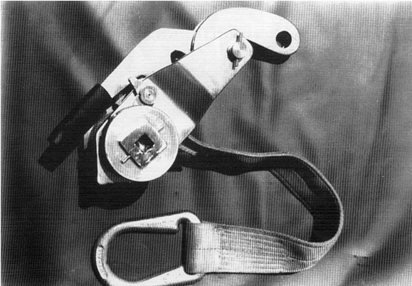
Webbing Assembly
